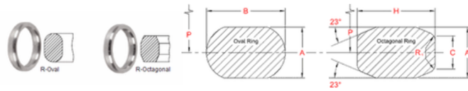
DIMENSIONAL DATA - R TYPES
